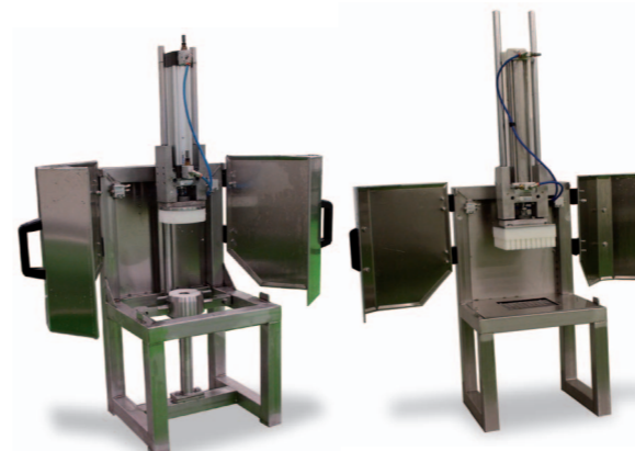
Fructus I - III Cutting machines
